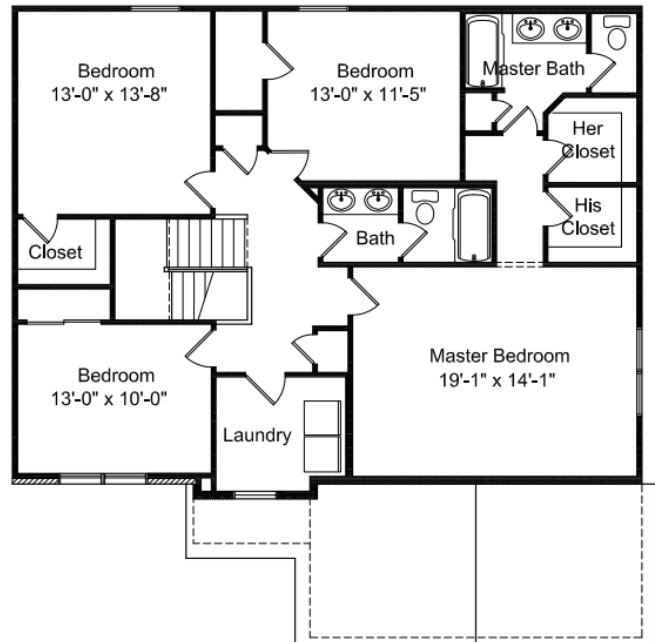
Second Floor Plan 1,363 Sq. Ft.
