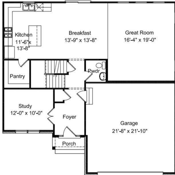
First Floor Plan 1,098 Sq. Ft.
