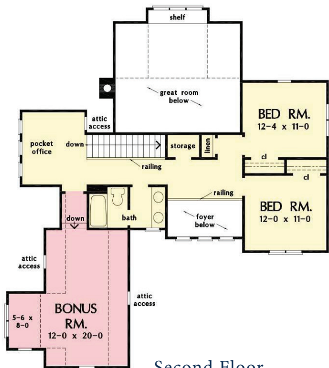
Second Floor
